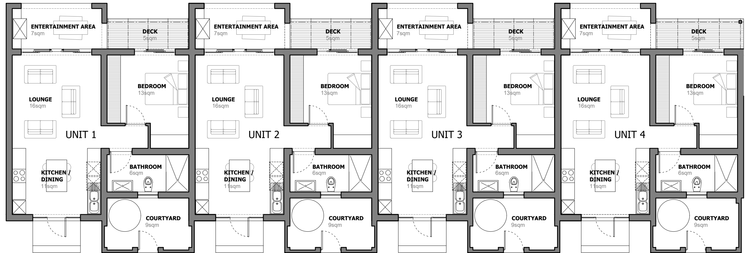
GARDEN COTTAGES (66sqm/unit) SCALE 1:50
